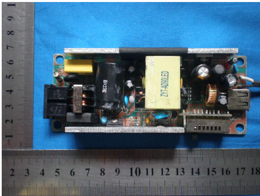
Photo 4 PCB component side
