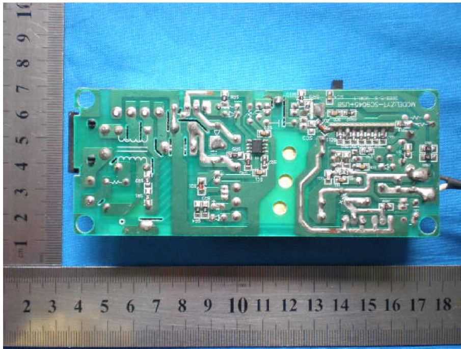
Photo 5 PCB component bottom
